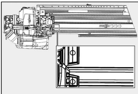
Fig. 1: Positioning the machine on the guiding device
