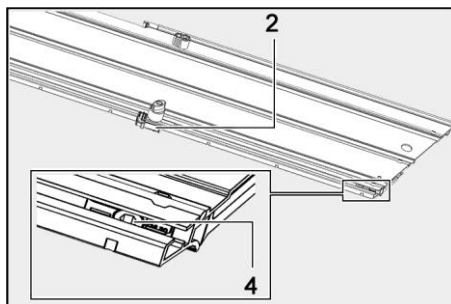
Fig. 7: Setting the repetition guide fence
