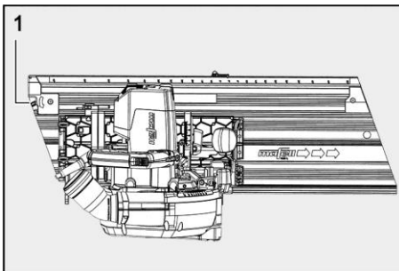
Fig. 2: Connecting the machine with the guiding device
