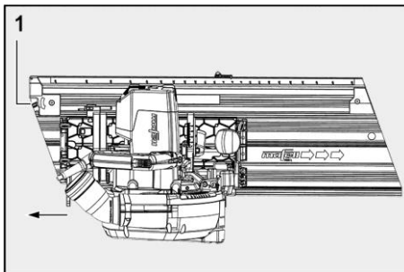
Fig. 3: Detaching the machine from the guiding device
