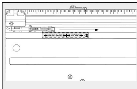
Fig. 17: Cleaning the spring guide
